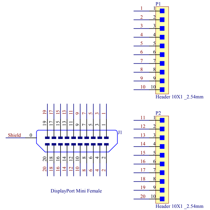
mDP-F-BO-V1A Schematic Diagram
